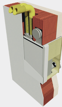
INTEGRATED INTO WALL U 2 VERSION WITH DUCTWORK CONNECTION
