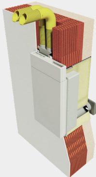
FLUSH-MOUNT VERSION WITH DUCTWORK CONNECTION
