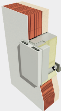
FLUSH-MOUNT VERSION
